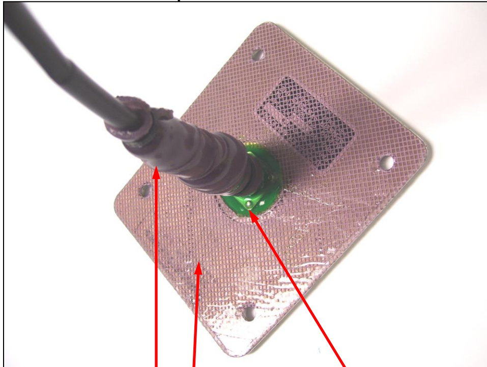
Figure 1 Typical HI-TAK® Non-Conductive Antenna Gasket Installation with HT3326-5 Self-Leveling Green® Sealant and StretchSeal™ Tape
